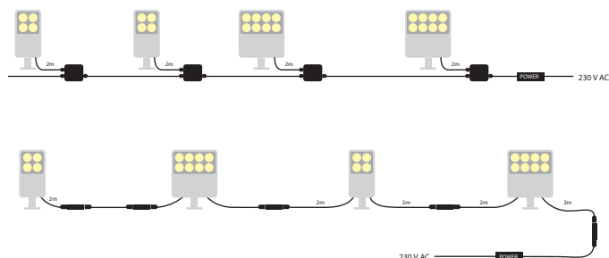
MONOCOLOR ON/OFF CONNECTIONS CONEXIONES ON/OFF MONOCOLOR
