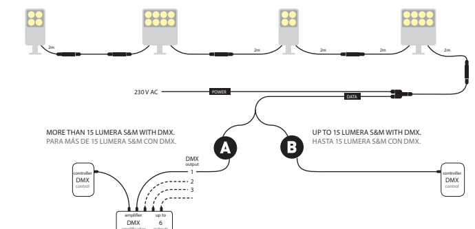
DMX CONNECTIONS CONEXIONES DMX
